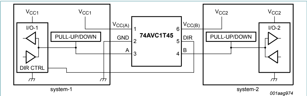
Fig. 9. Bidirectional logic level-shifting application
