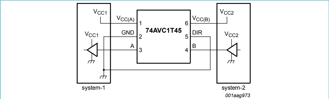
Fig. 8. Unidirectional logic level-shifting application
