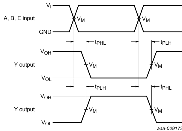
Fig. 3. Input A, B and E to output Y propagation delay times
