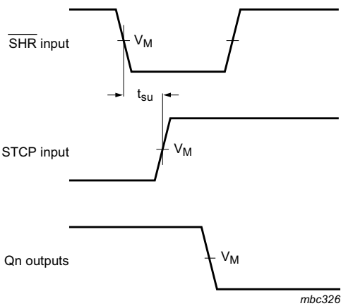
Fig 11. The set-up time shift reset ( \overline{\text{SHR}} ) to storage clock (STCP)
