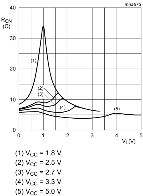
Fig. 8. Typical ON resistance as a function of input voltage; T_{amb} = 25\text{ °C}
