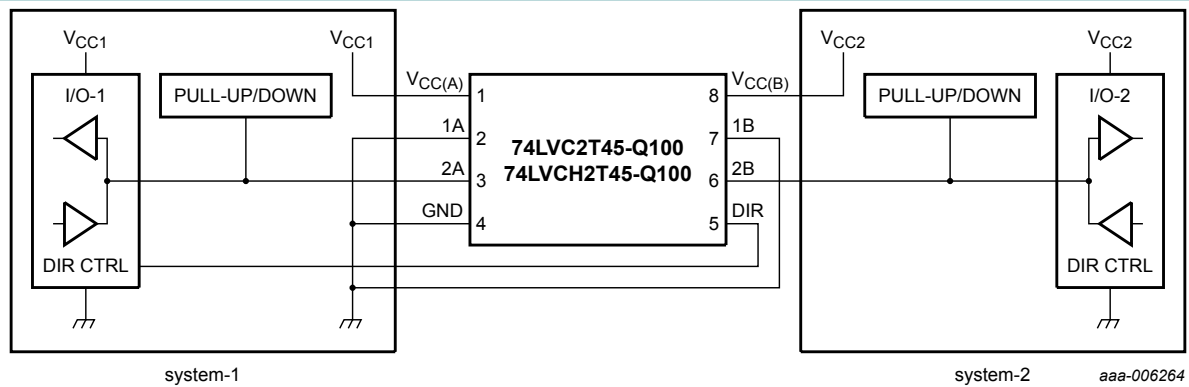
Fig. 15. Bidirectional logic level-shifting application
