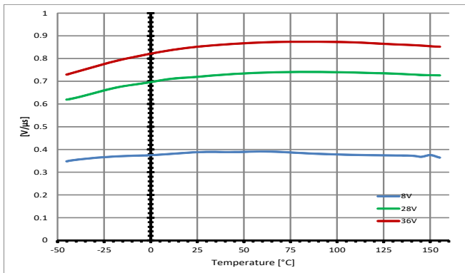
Slew Rate at Turn ON dV/dt_{ON} = f(T_J; V_S), R_L = 4 \Omega
