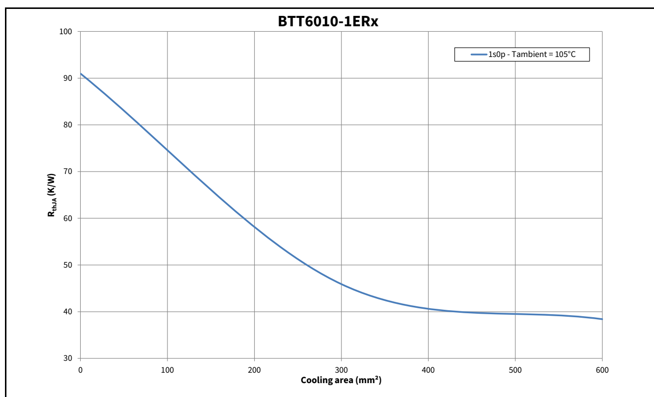
Figure 7 Typical Thermal Resistance. PCB set-up 1s0p
