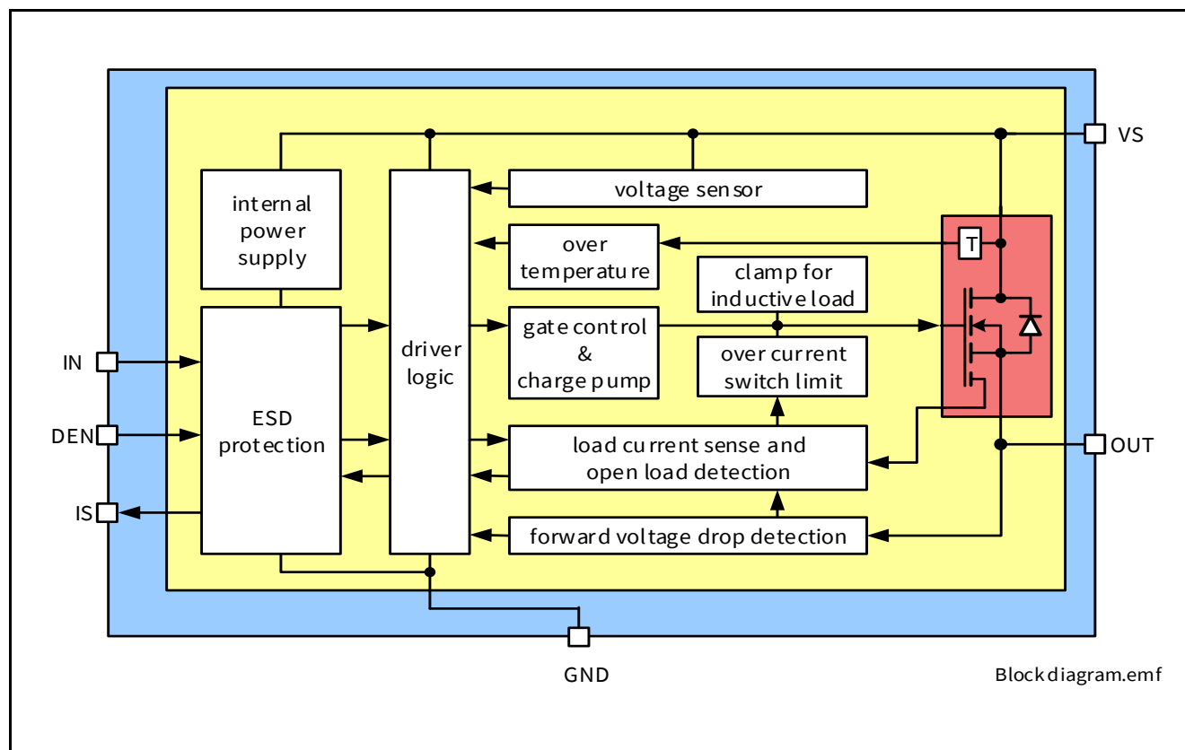
Figure 1 Block Diagram for the BTT6010-1ERA
