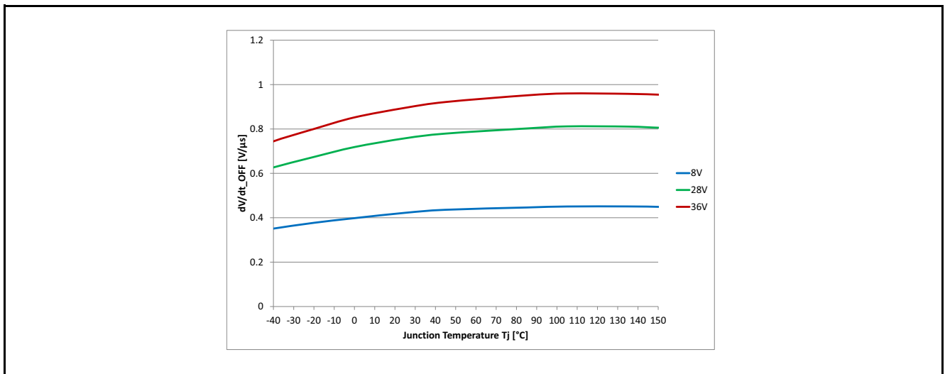
Figure 36 Slew Rate at Turn OFF - dV/dt_{OFF} = f(T_J; V_S) , R_L = 12 \Omega
