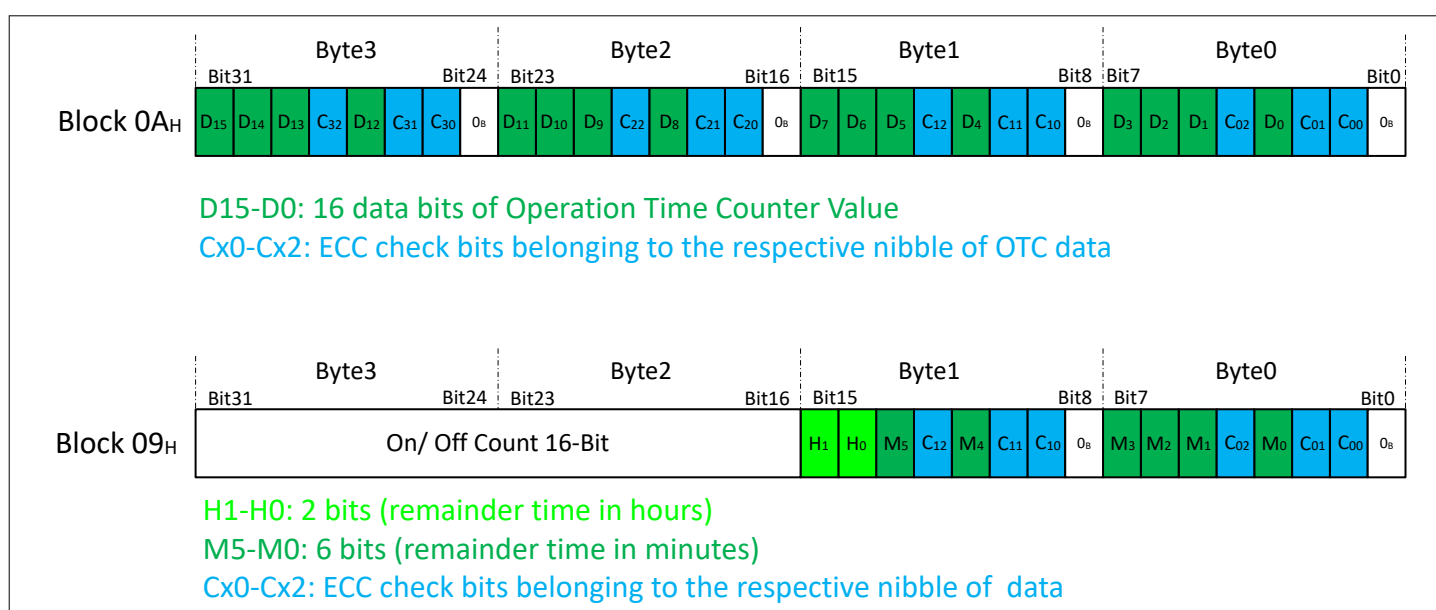
Figure 13 OTC related NVM content
