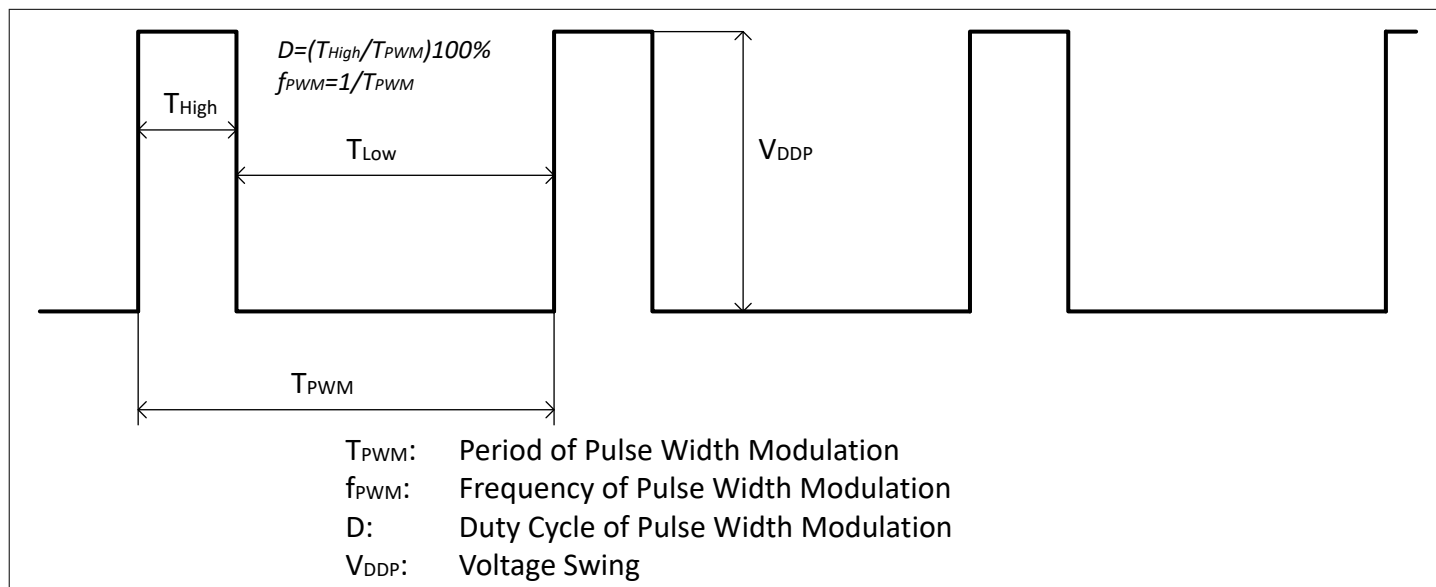
Figure 14 PWM Output Characteristics
