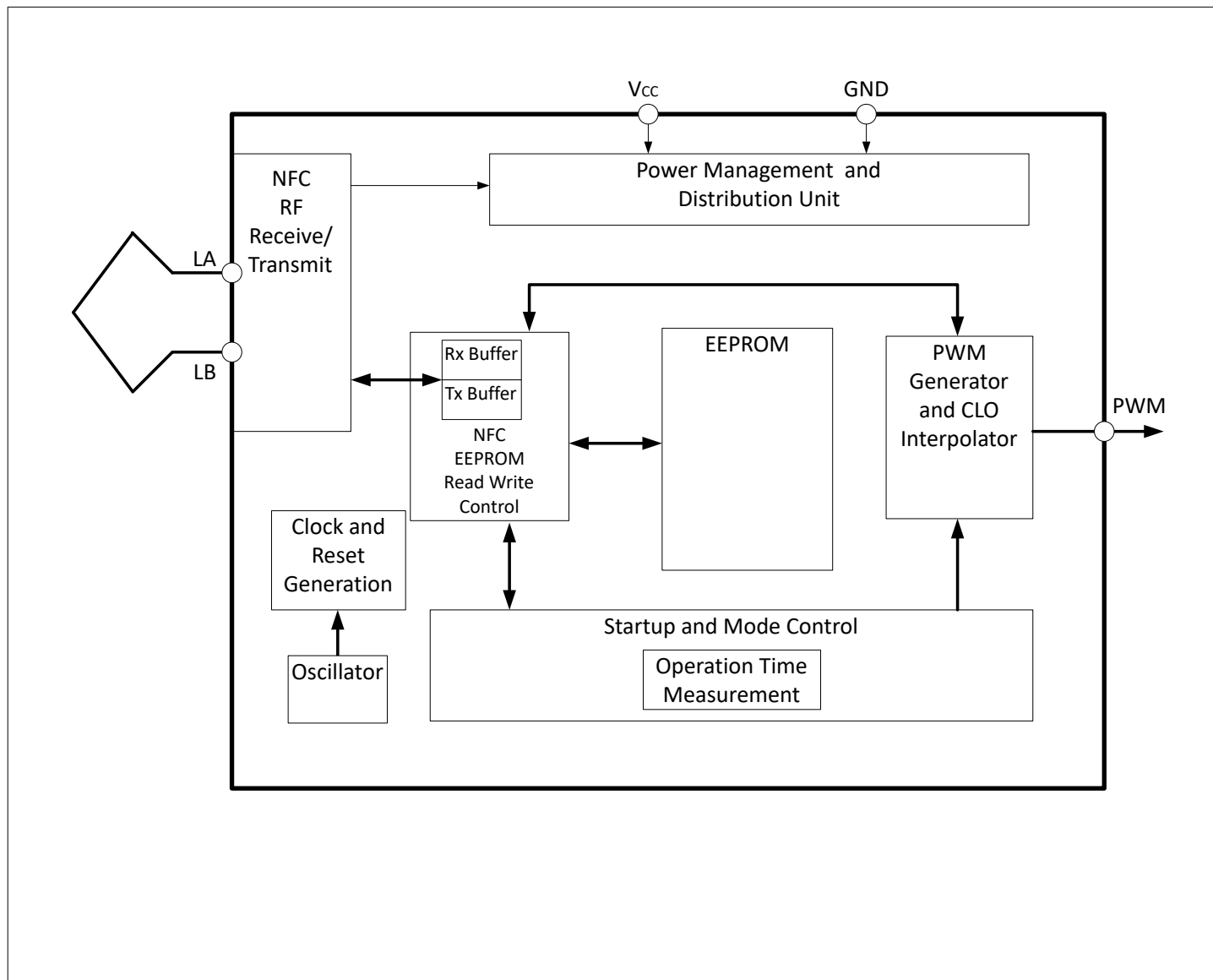
Figure 3 Block Diagram
