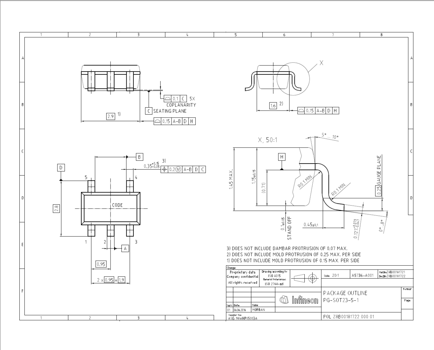
Figure 15 Package Outline PG-SOT23-5-1
