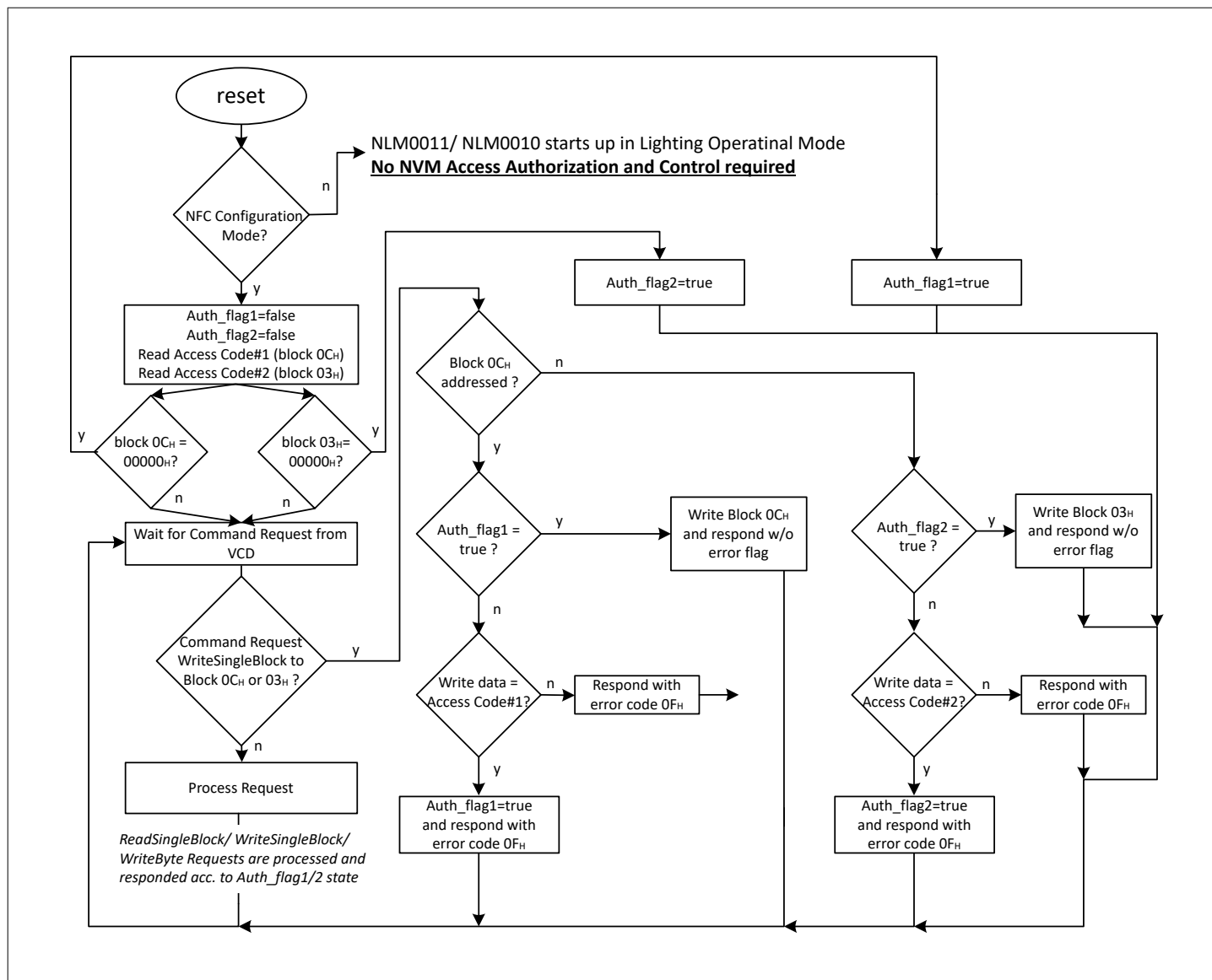
Figure 8 Access Authorization Flow Chart
