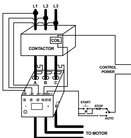
CURRENT TRANSFORMER WIRING DIAGRAM OR MODEL 777-ACCUPOWER
