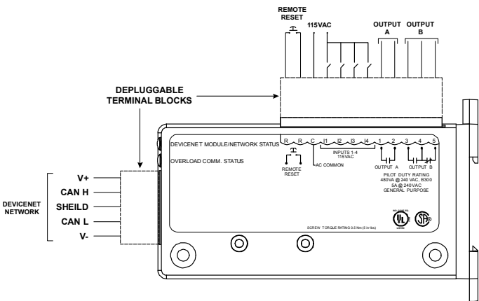
TYPICAL WIRING FOR CIO-120-DN-P
