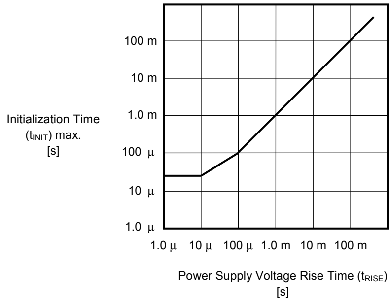
Figure 27 Initialization Time of S-24C128C
