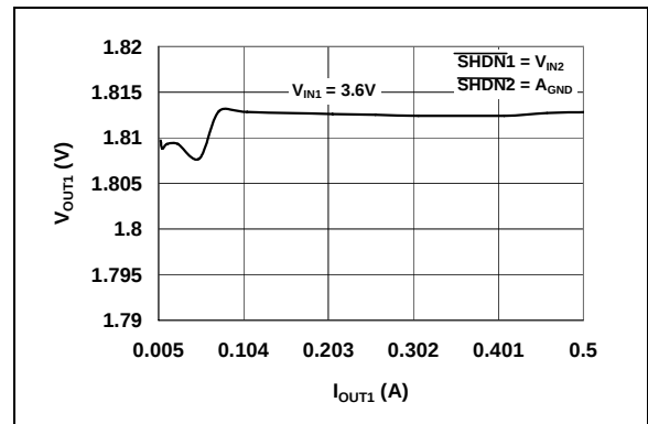
FIGURE 2-12: V_{OUT1} vs. I_{OUT1} ( V_{OUT1} = 1.8V ).
