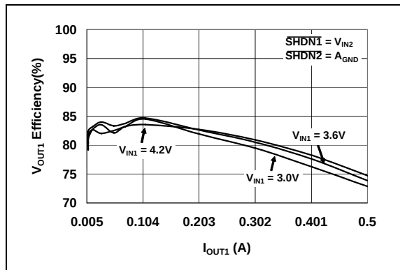
FIGURE 2-6: V_{OUT1} Output Efficiency vs. I_{OUT1} ( V_{OUT1} = 1.2V ).
