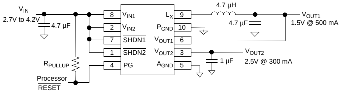
TC1303A Fixed-Output Application 10-Lead MSOP
