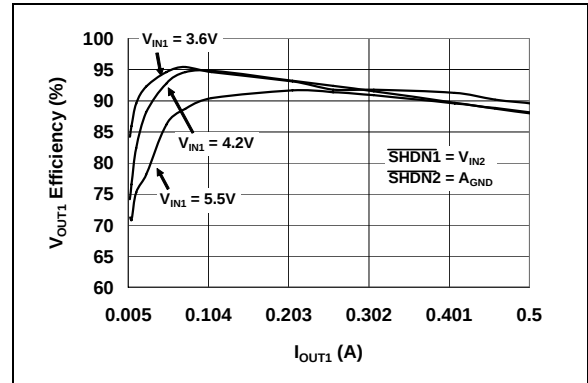
FIGURE 2-10: V_{OUT1} Output Efficiency vs. I_{OUT1} ( V_{OUT1} = 3.3V ).
