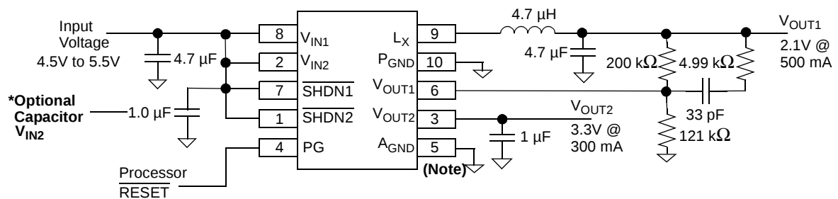
TC1303B Adjustable-Output Application 10-Lead DFN
