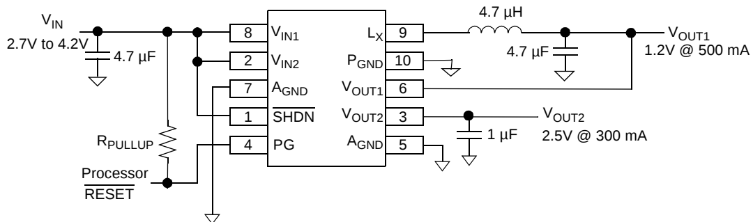
TC1304 Fixed-Output Application 10-Lead MSOP
