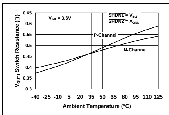
FIGURE 2-18: V_{OUT1} Switch Resistance vs. Ambient Temperature.
