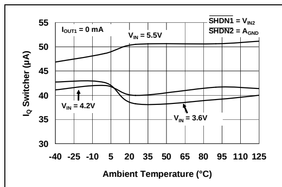
FIGURE 2-3: I_Q Switcher Current vs. Ambient Temperature.
