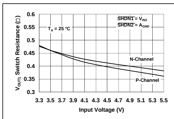
FIGURE 2-17: V_{OUT1} Switch Resistance vs. Input Voltage.
