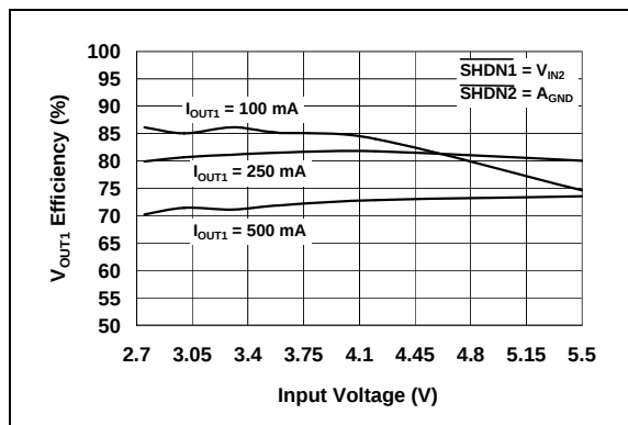
FIGURE 2-5: V_{OUT1} Output Efficiency vs. Input Voltage ( V_{OUT1} = 1.2V ).
