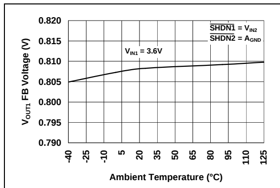
FIGURE 2-16: V_{OUT1} Adjustable Feedback Voltage vs. Ambient Temperature.
