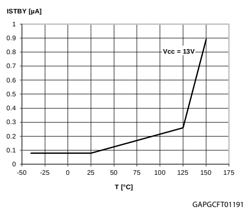
Figure 16: Standby current
