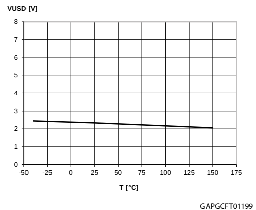
Figure 24: Undervoltage shutdown
