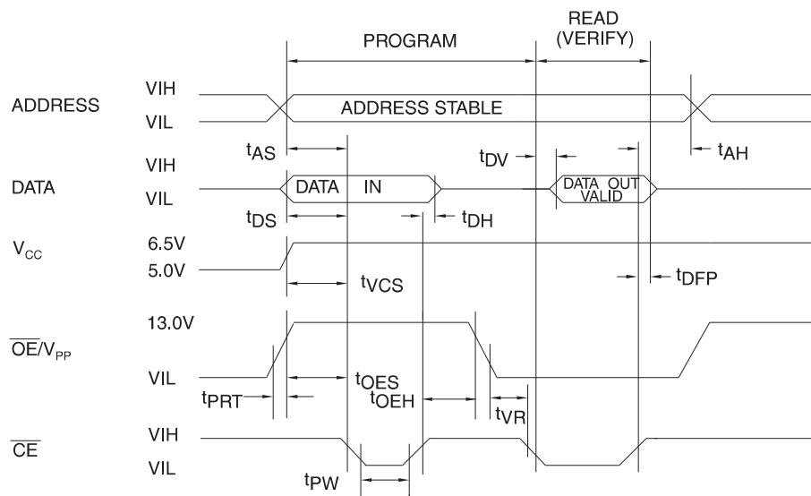
Figure 5-4. Programming Waveforms (1)
