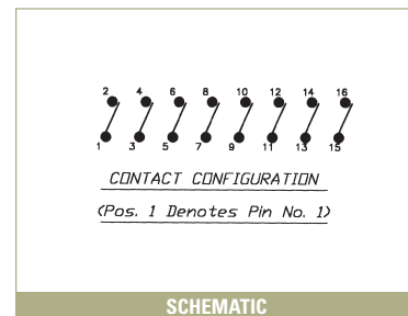
SCHEMATIC
