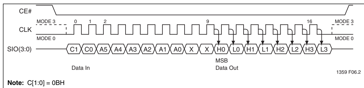
Figure 11: High-Speed Read Sequence (SQI)
