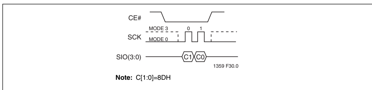
Figure 24: Lockdown Block-Protection Register
