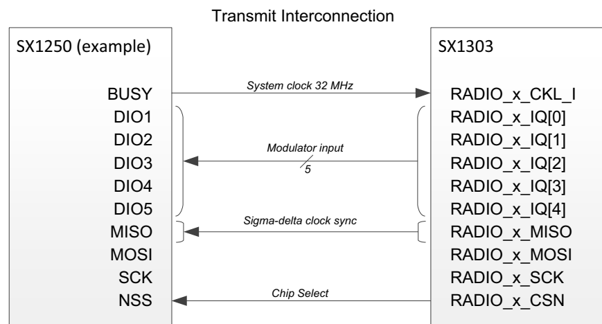
Figure 4-2: Transmit Interconnection
