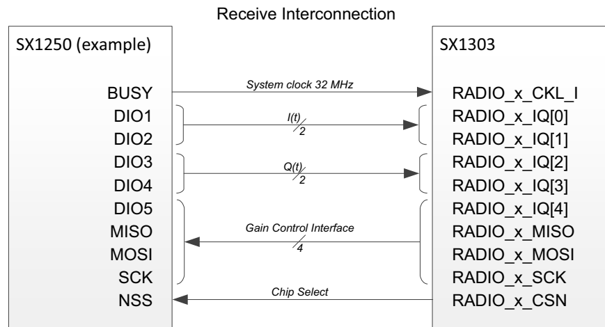
Figure 4-1: Receive Interconnection
