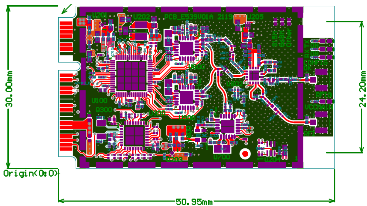
Figure 10-2: Reference Design PCB Layout
