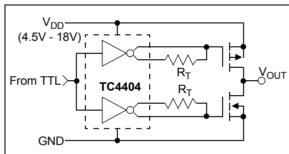
FIGURE 4-2: Zero Crossover Current Totem-Pole Switch.
