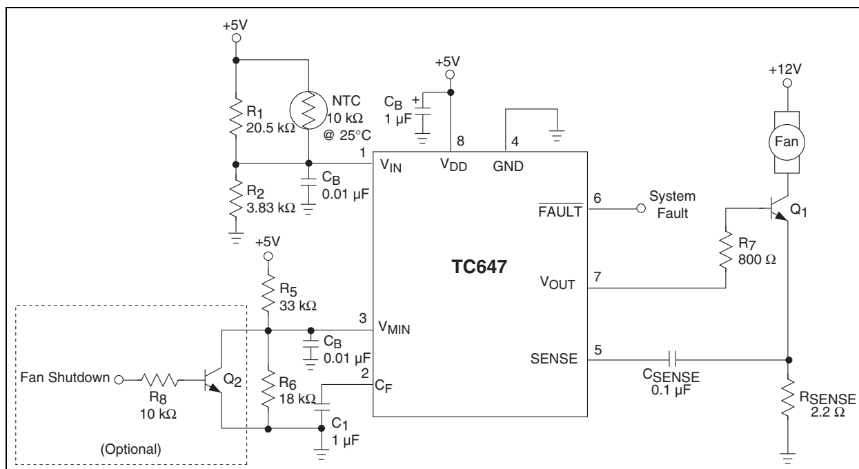
FIGURE 5-9: Design Example.
