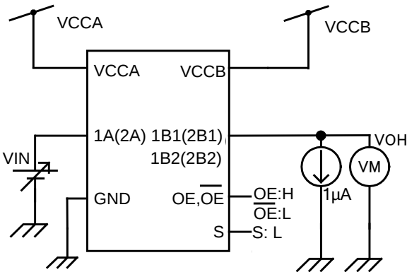
Figure 9 Test Circuit
