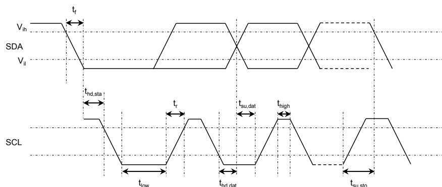
Figure 6. I 2 C timing diagram
