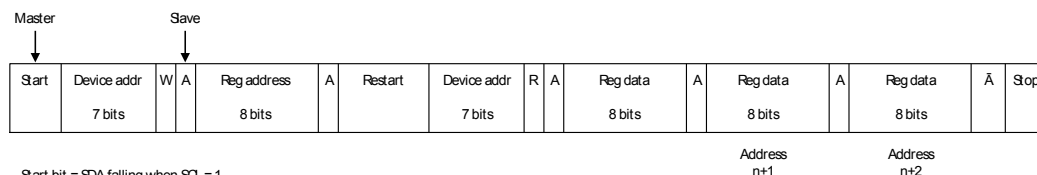
Figure 4. Read operation
